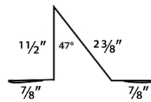
Snow Fence
