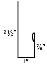
J-Channel
