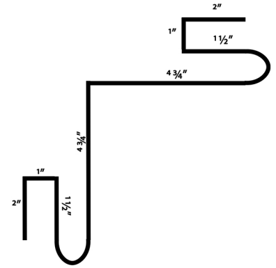
Inside Corner/ J-Channel Combo
