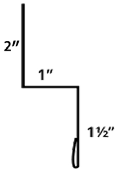
Double Angle
