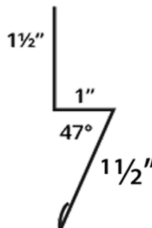
Wall Base
