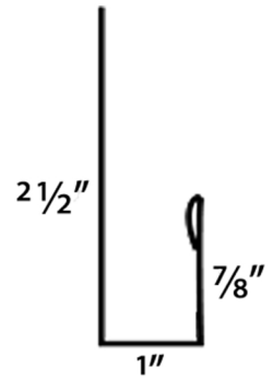
J-Channel
