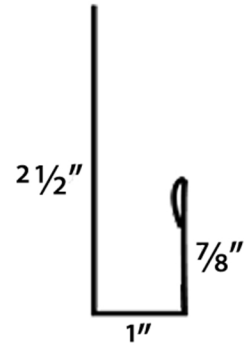
J-Channel
