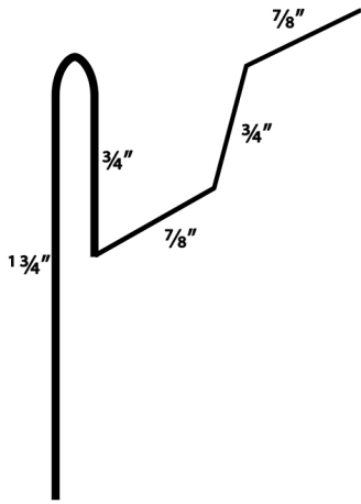
Starter Strip
