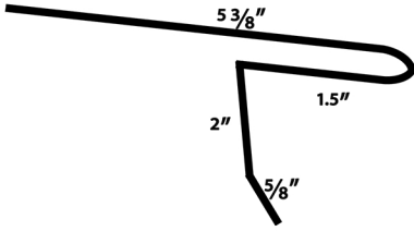
Roof Starter
