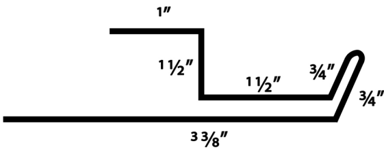
J-Z Combo
