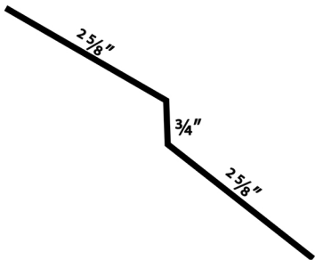
Cleat
