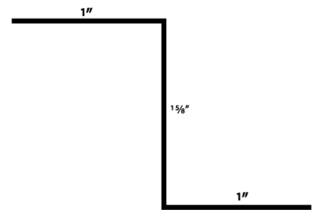
Z-Bar
