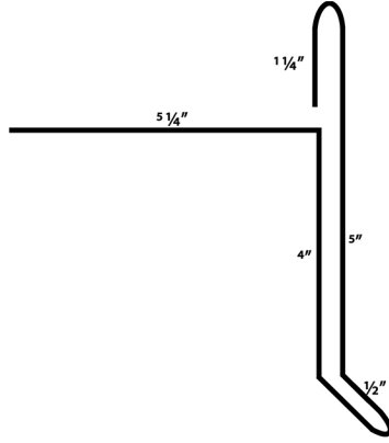
Starter Rake
